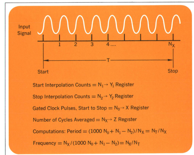
Fig. 3. For period and frequency measurements the computing counter's measurement cycle is synchronized with the input signal. The selected measurement time is actually a minimum value; the actual time is an integral number of input periods. Besides measuring T_0 , T_1 , and T_2 as for time interval, the counter counts the input periods N_X and then computes period or frequency.
