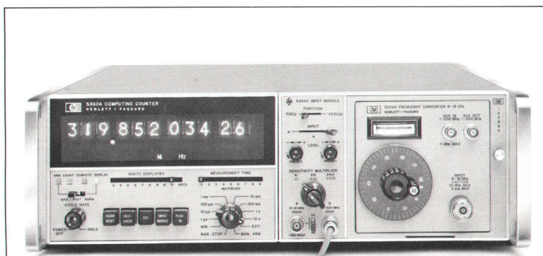
Fig. 1. Model 5360A Computing Counter is orders of magnitude more powerful than earlier counters. It measures CW or pulsed carrier frequencies between 0.01 Hz and 320 MHz to as many as 11 significant digits. Frequency-converter plug-ins extend its range to 18 GHz. It measures period (and time interval with another plug-in) with 1 ns accuracy and 0.1 ns resolution.
