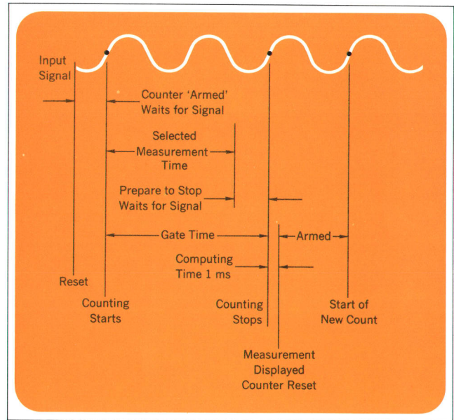
Fig. 4. The automatic counter's measurement cycle is always synchronized with the input signal. The selected measurement time is actually a minimum value.
